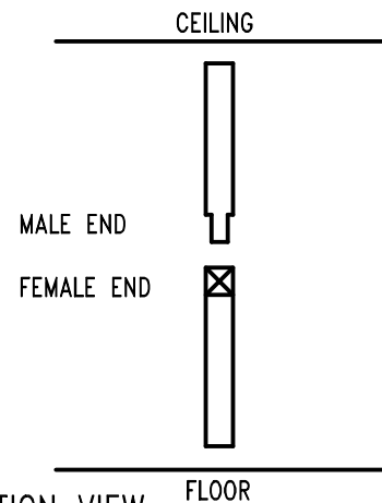
ELEVATION VIEW
